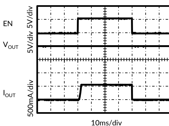
Figure 18. Device Enabled into Short-Circuit
