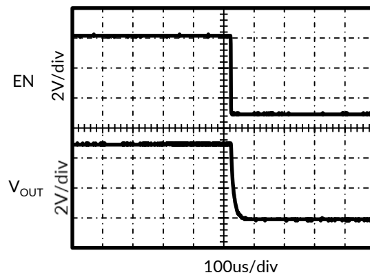
Figure 16. Turn-Off Delay Time
