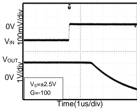
Figure 15. Positive Overload Recovery
