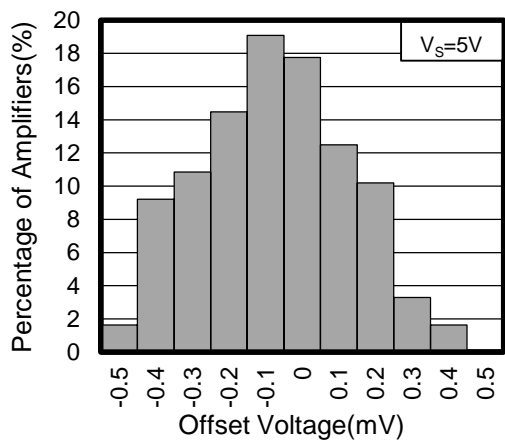
Figure 17. Offset Voltage Production Distribution
