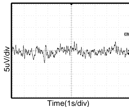
Figure 12. 0.1Hz to 10Hz Input Voltage Noise
