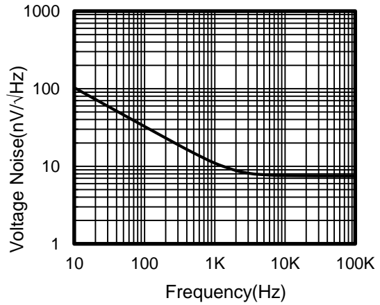
Figure 2. Input Voltage Noise Spectral Density vs Frequency
