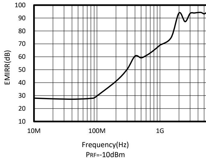
Figure 19. RS62XP EMIRR vs Frequency
