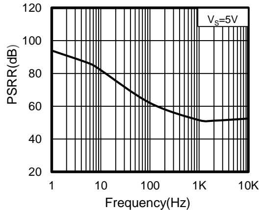
Figure 4. Power-Supply Rejection Ratio vs Frequency
