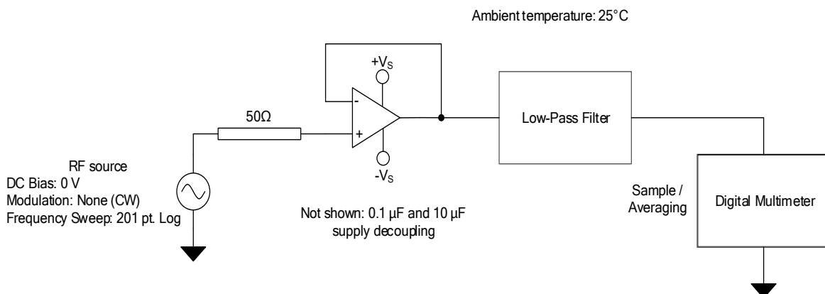
Figure 20. EMIRR IN+ Test Configuration Schematic
