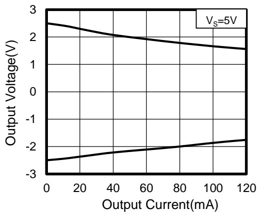
Figure 13. Output Voltage vs Output Current
