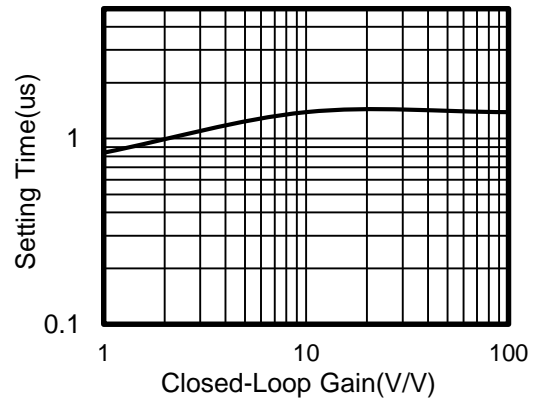
Figure 12. Setting Time vs Closed-loop Gain
