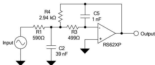
Figure 21. 25-kHz Low-Pass Filter
