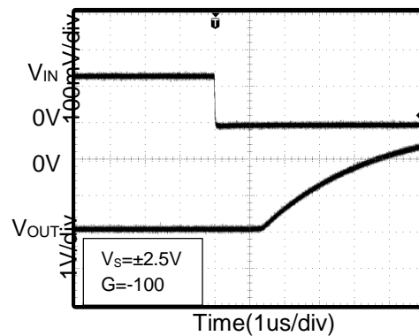
Figure 16. Negative Overload Recovery
