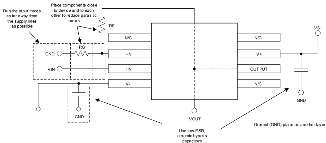
Figure 24. Operational Amplifier Board Layout for Noninverting Configuration
