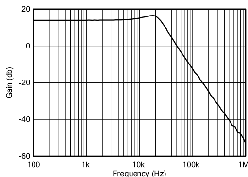
Figure 22. Low-pass filter transfer function
